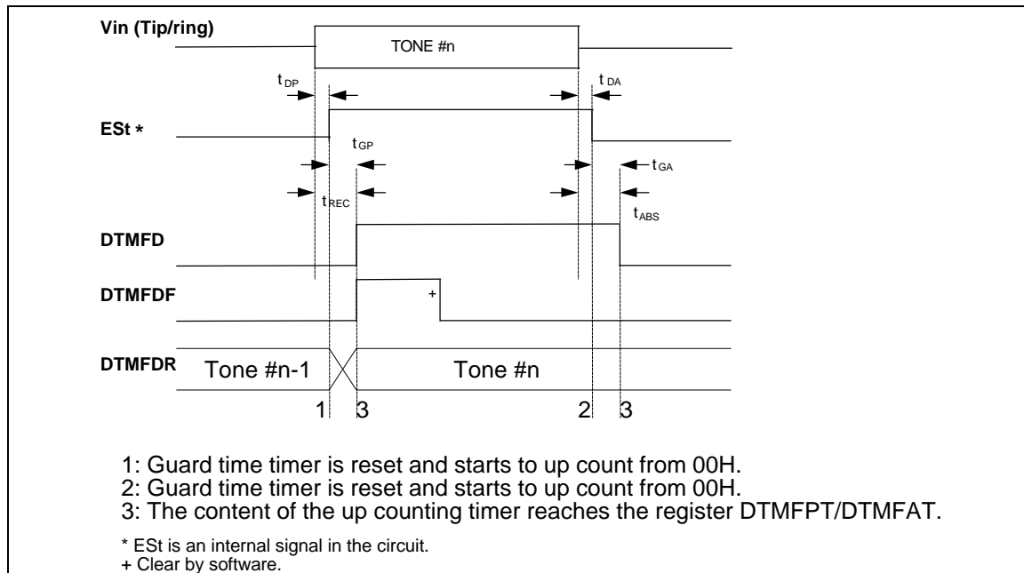
Figure 6-22 The Waveform of DTMF Detection
