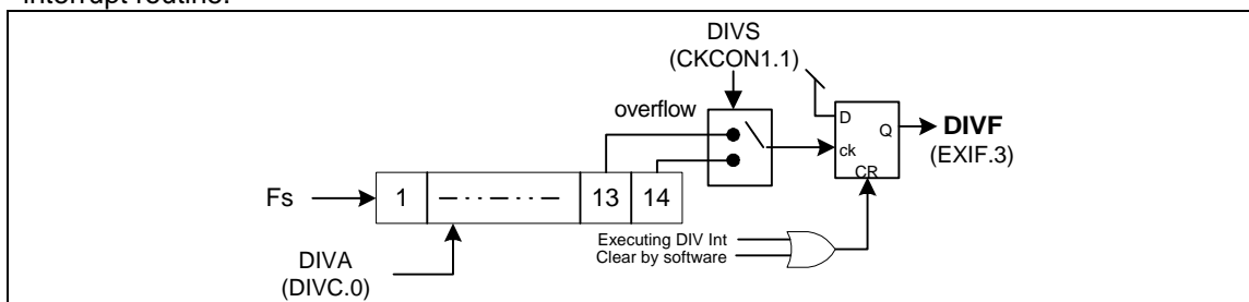
Figure 6-13 13/14-bit Divider
