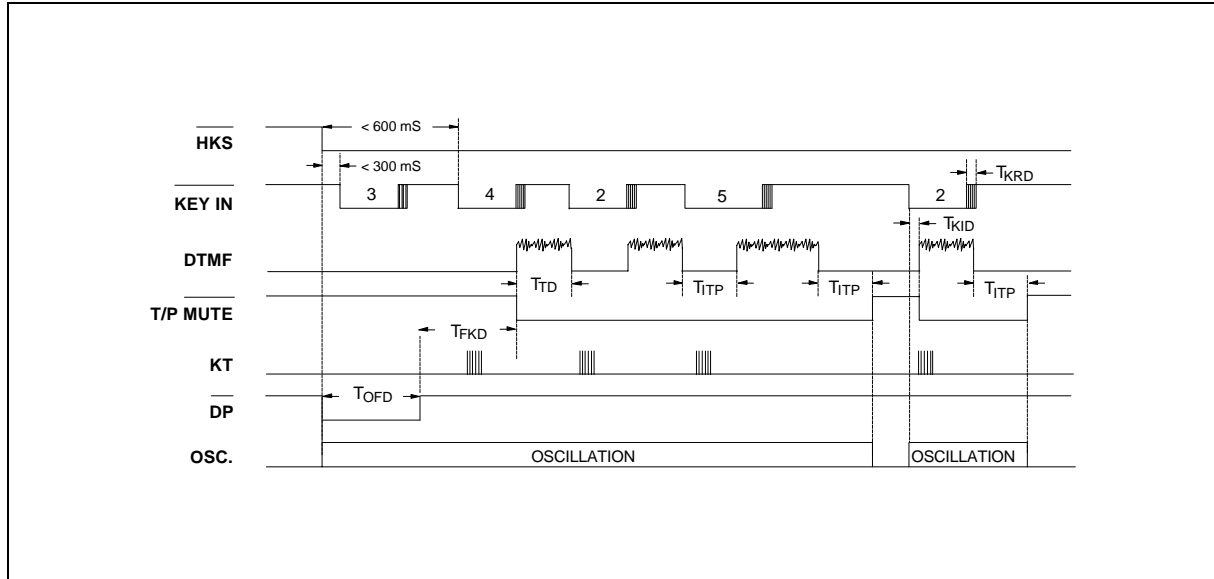
Timing Waveforms, continued
