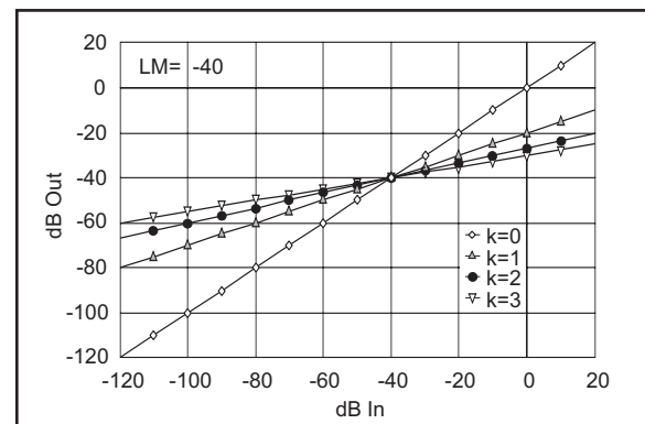
Figure 8. Compressor input-output transfer characteristics with varying k .
