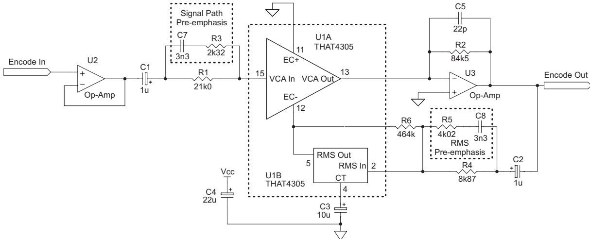
Figure 20. 4305 hi-fi 2:1 encoder circuit
