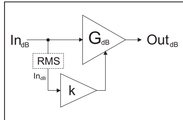
Figure 5. Simplified feedforward expander, conceptual diagram
