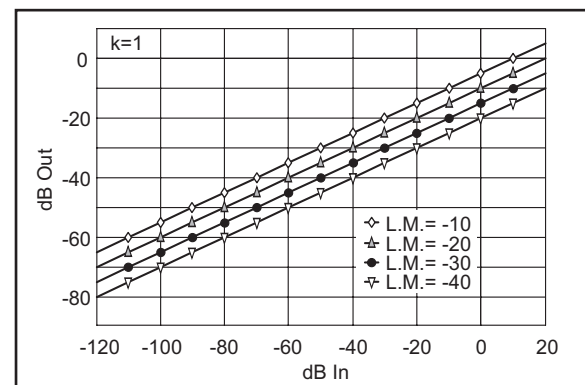
Figure 9. Compressor input-output transfer characteristics with varying LM_{dB}
