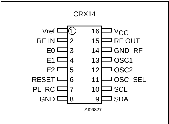
Figure 3. SO Connections
