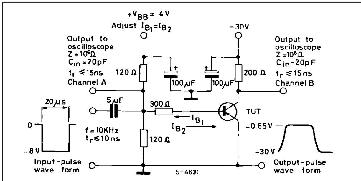
Test Circuit for t_{on} , t_{off} .
