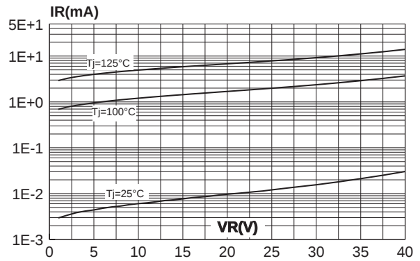
Fig. 6-2: Reverse leakage current versus reverse voltage applied (typical values) (1N5822).
