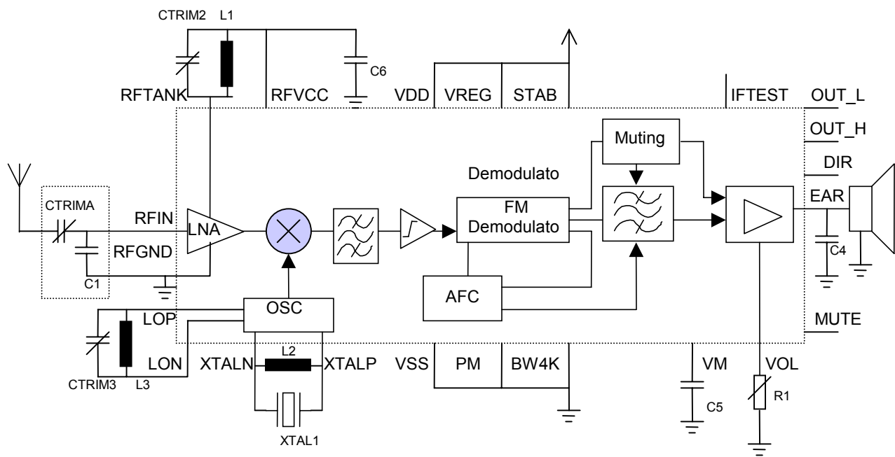
Components list for F=171 MHz
