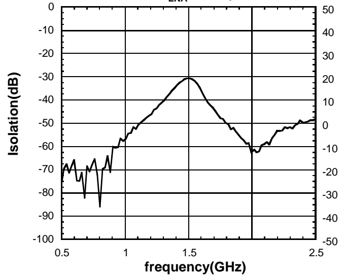
RF OUT-MIXER IN Isolation
