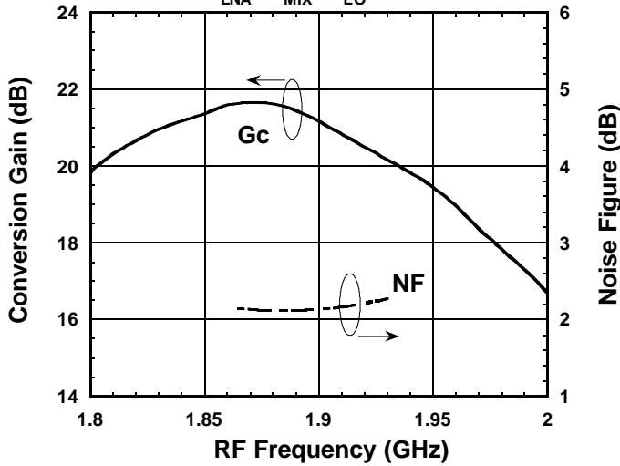
Conversion Gain , Noise Figure vs. RF Frequency (V_{LNA}=V_{MIX}=V_{LO}=2.7V)
