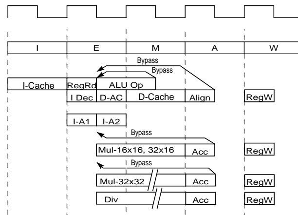
Figure 2 4KEm Core Pipeline
