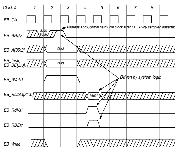
Figure 7 Single Read Transaction Timing Diagram
