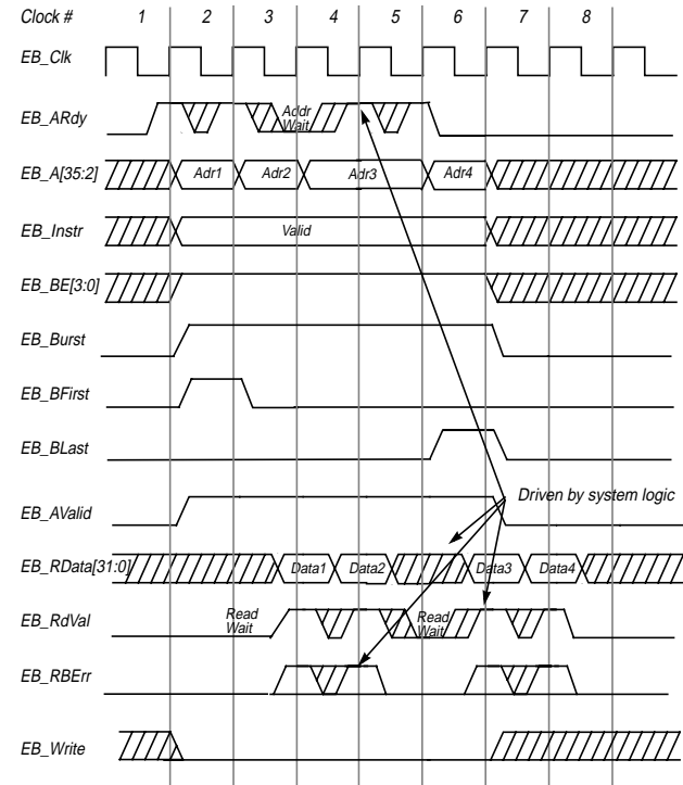
Figure 10 Burst Read Transaction Timing Diagram
