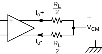
Figure 9.1 LVD Driver
