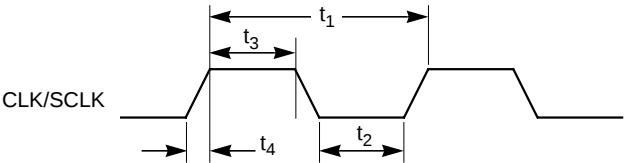
Figure 9.8 LSI53C040 Clock Waveforms
