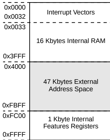
Figure 2.2 LSI53C040 Memory Map
