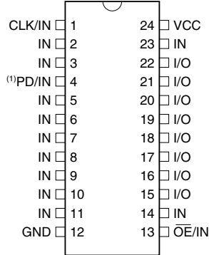
DIP/SOIC
