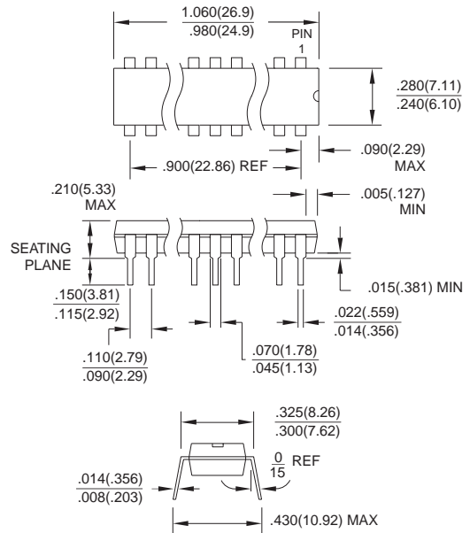
20P3 , 20-Lead, 0.300" Wide, Plastic Dual Inline Package (PDIP) Dimensions in Inches and (Millimeters) JEDEC STANDARD MS-001 AD
