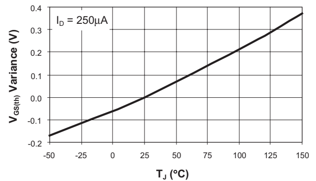
Threshold Voltage
