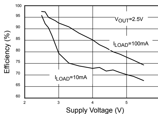
Fig. 10 Efficiency vs. Input Voltage
