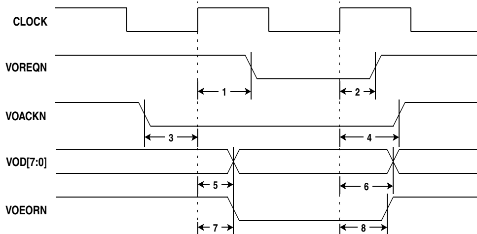
Figure 22: Video Output Port Timing
