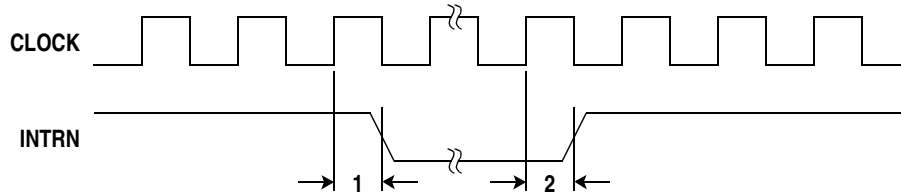
Figure 25: Interrupt Timing
