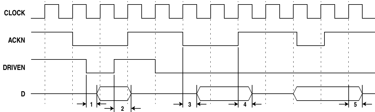
Figure 21: Output Enable Timing
