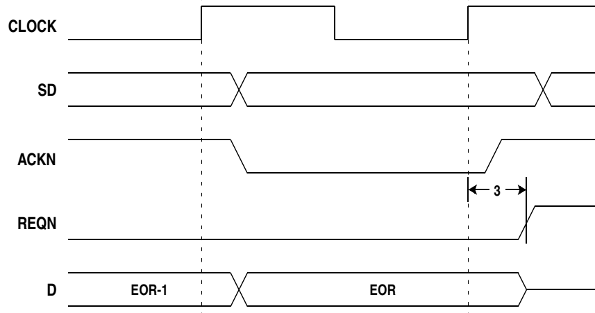
Figure 18: Request Deasserts at EOR, Strobe Condition of DSC=0-3, 6-15; ERC=1
