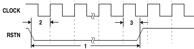
Figure 27: Power On Reset Timing
