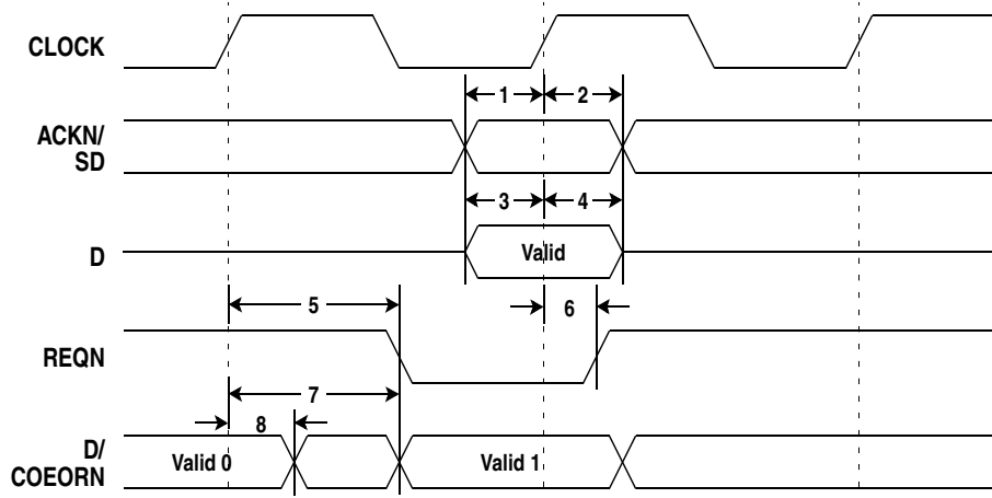
Figure 16: Data Interface Timing
