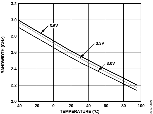
Figure 6. Bandwidth vs. VCC and Temperature
