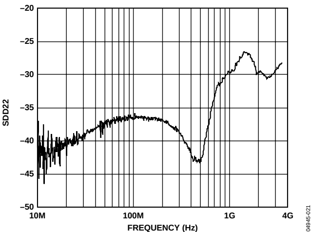
Figure 8. SDD22 vs. Frequency up to 3.5 GHz, CAP = Open
