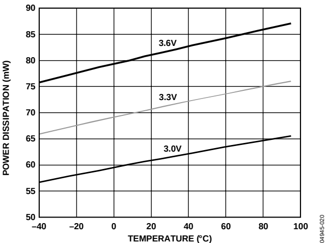
Figure 7. Power Dissipation vs. VCC and Temperature
